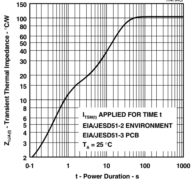
THERMAL IMPEDANCE vs POWER DURATION
