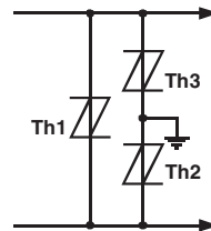
Figure 13. Multi-point Protection
