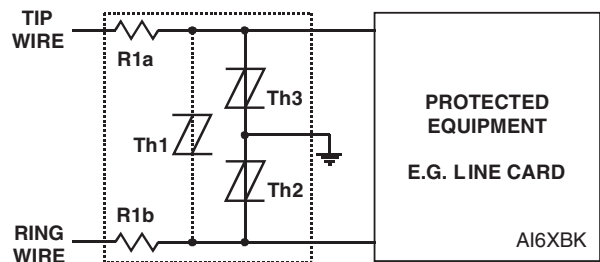
Figure 15. Protection Module
