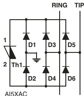
Figure 14. Low Capacitance Bridge Protection Circuit
