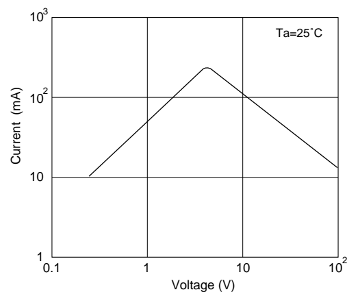
Current - Voltage Characteristics (Static Characteristics)
