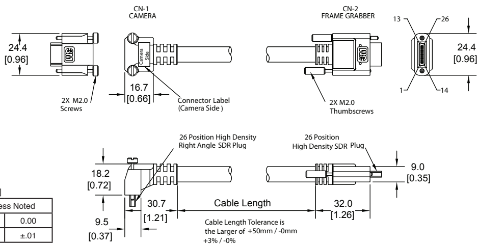
Figure 2 Straight SDR - Right-Angle SDR 1SD26-X13X-00C-XXX
