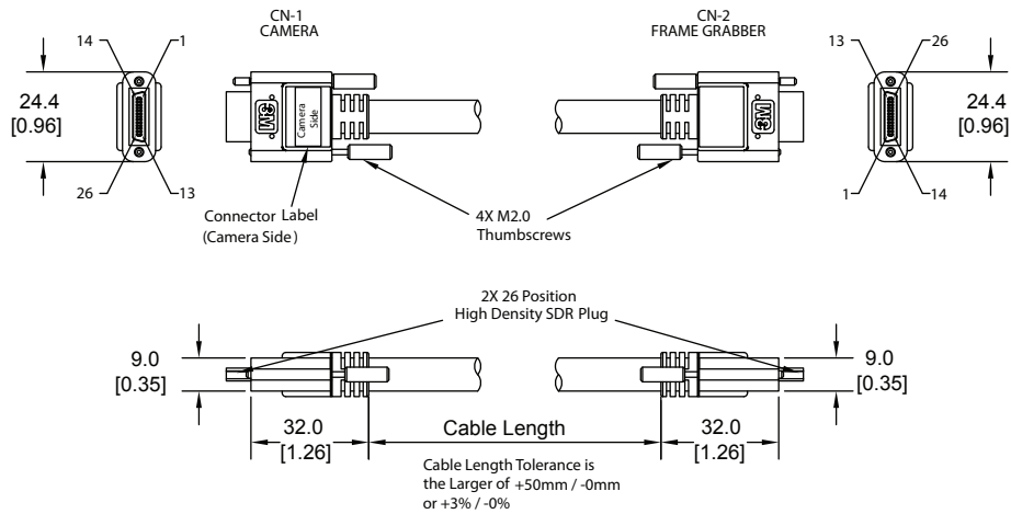
Figure 1 Straight SDR - Straight SDR 1SD26-X120-00C-XXX
