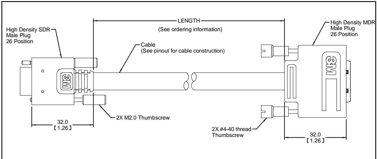
Figure 1 MDR Straight To SDR Straight Cable Assembly
