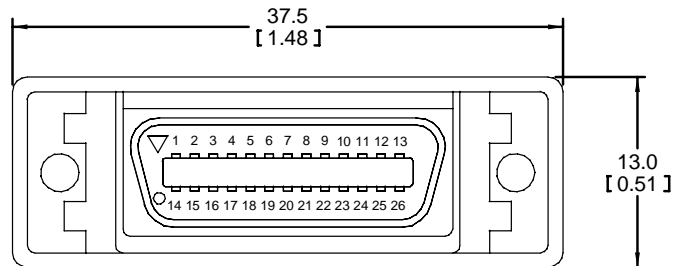
Figure 3 MDR Plug Pinout
