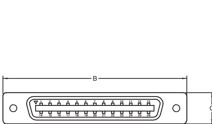
Generic End Detail MDR 26 Position Plug (Both Ends)
