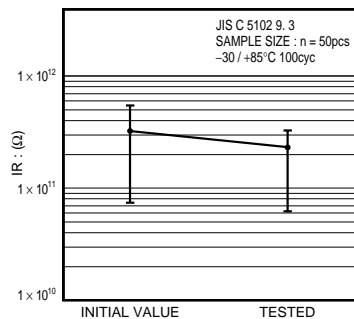
Fig.15 Insulation resistance
