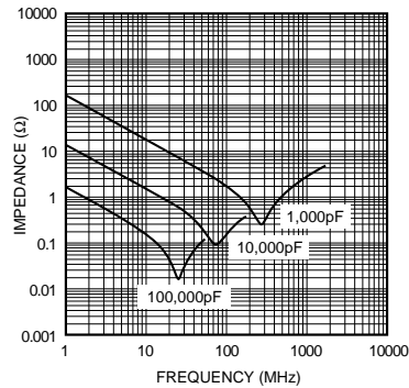
Fig.6 Impedance-frequency characteristics
