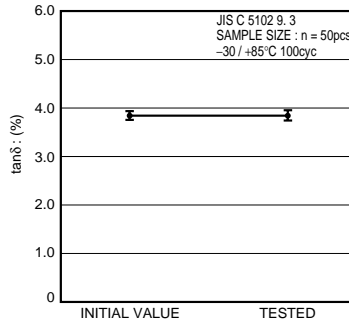
Fig.14 tanδ
