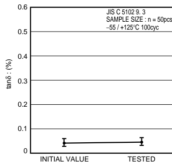
Fig.8 tanδ
