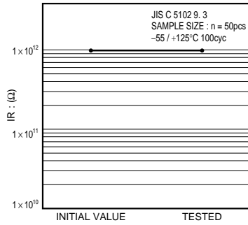
Fig.9 Insulation resistance
