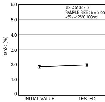
Fig.11 tanδ
