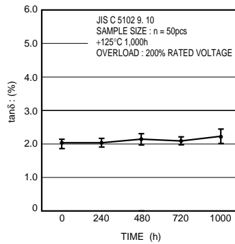
Fig.20 tanδ
