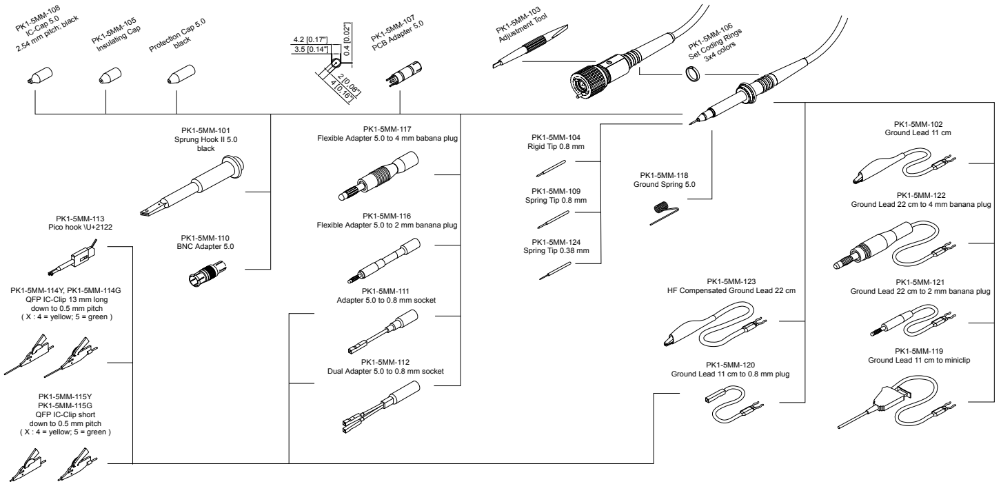
Probe Accessory Diagram for PP005A, PP009 and PP011 Passive Probes
