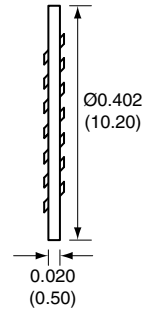
WASHER
