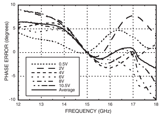
Phase Error vs. Frequency, Fmean = 15 GHz [1]
