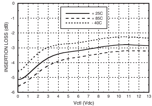
Insertion Loss vs. Vctl , F = 15 GHz
