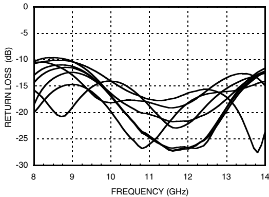
Input Return Loss, Major States Only
