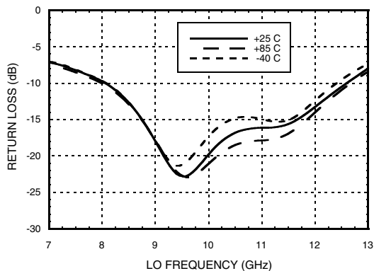
LO Return Loss vs. Temperature
