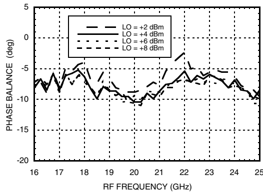
Phase Balance vs. LO Drive [1]
