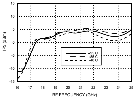
Input IP3, USB vs. Temperature
