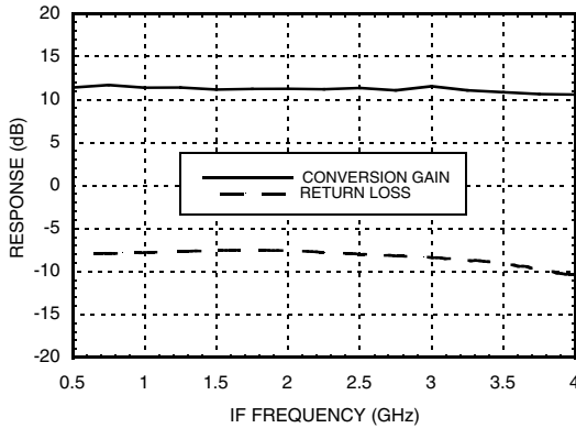
IF Bandwidth
