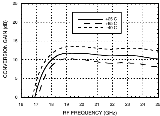
Conversion Gain, USB vs. Temperature
