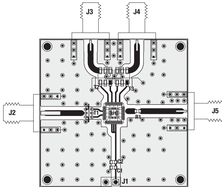
Component Placement
