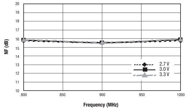
Figure 8. Noise Figure vs Frequency and Supply Voltage @ 900 MHz
