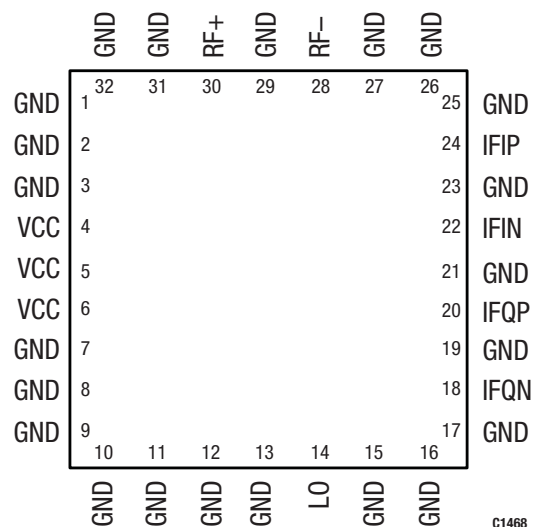
Figure 2. SKY73012 Pinout– 32-Pin RFLGA Package (Top View)
