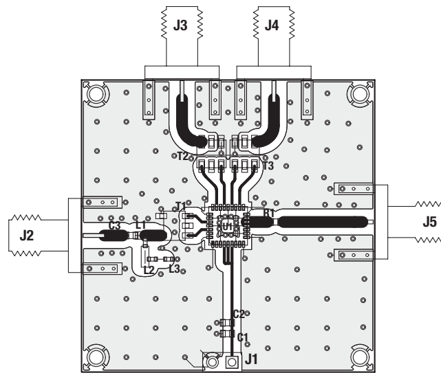
Component Placement
