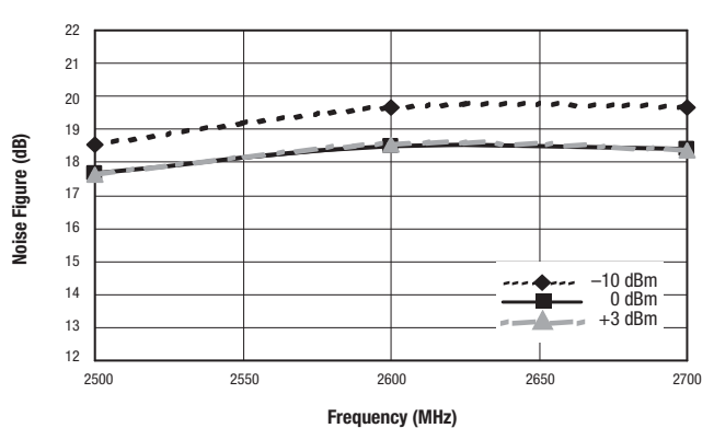
Figure 44. Noise Figure vs Frequency and LO Power @ 2600 MHz
