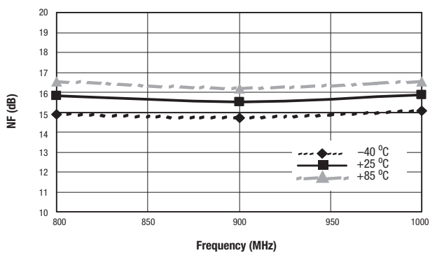
Figure 7. Noise Figure vs Frequency and Temperature @ 900 MHz
