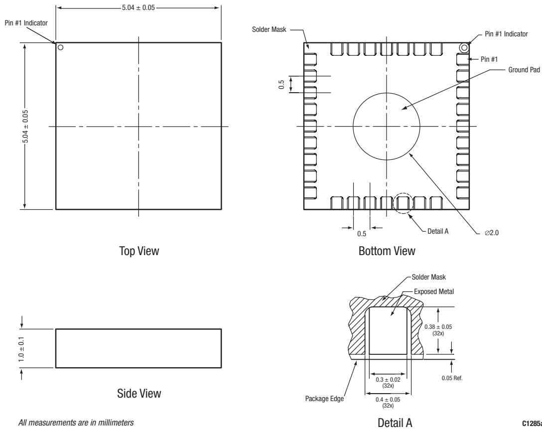
Figure 67. SKY73012 32-Pin RFLGA Package Dimensions
