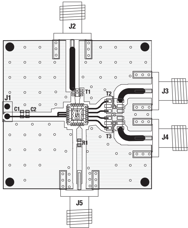
Component Placement
