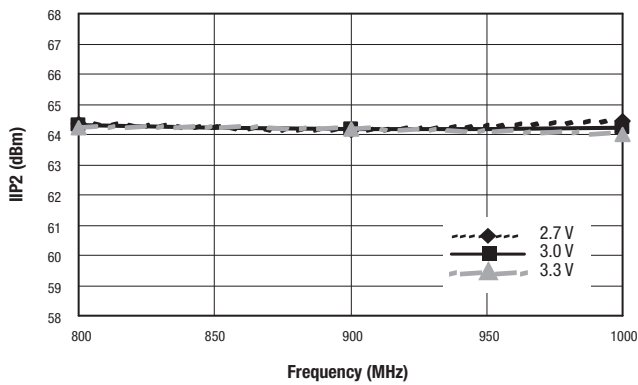
Figure 11. IIP2 vs Frequency and Supply Voltage @ 900 MHz
