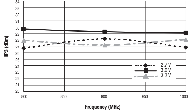
Figure 14. IIP3 vs Frequency and Supply Voltage @ 900 MHz
