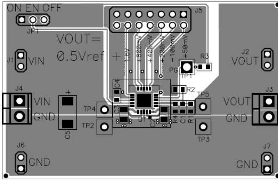
Figure 3. Assembly Layer
