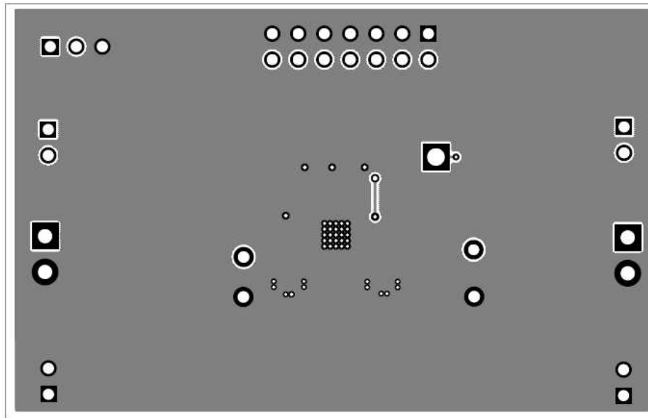
Figure 5. Bottom Layer Routing
