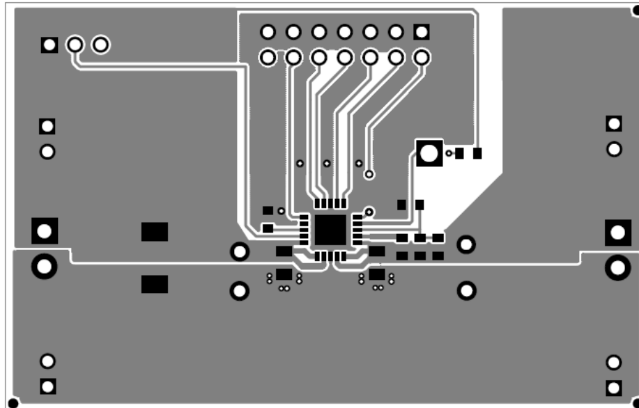
Figure 4. Top Layer Routing
