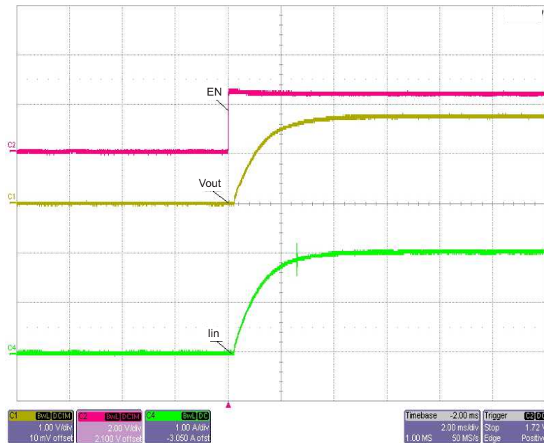
Figure 1. Turnon Sequence
