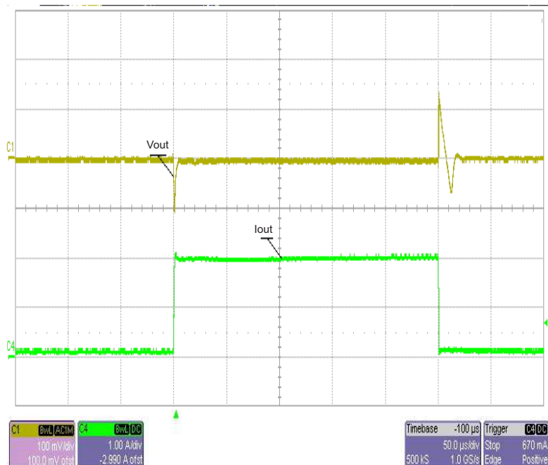
Figure 2. Step-Load and Output Voltage Transient Response
