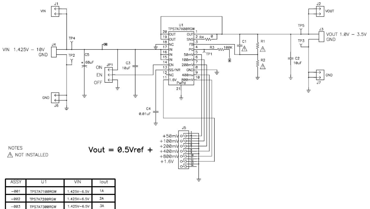
Figure 6. TPS7A7x00EVM-718 Schematic
