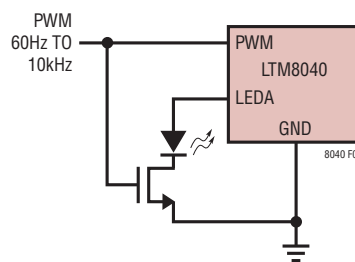
Figure 5. Dimming Using PWM Signal
