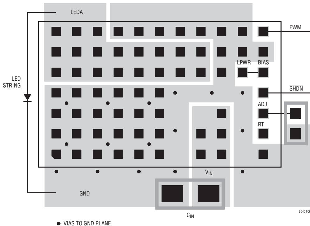
Figure 6. Suggested Layout
