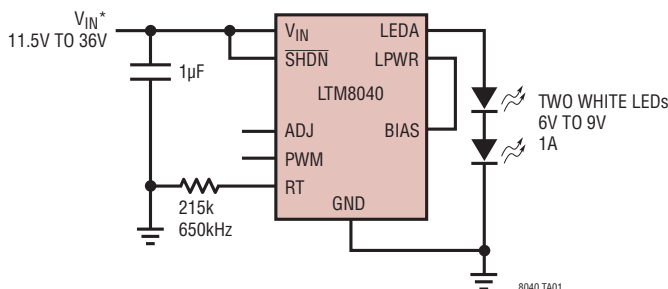
1A \mu Module LED Driver
