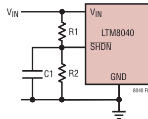
Figure 1. Undervoltage Lockout
