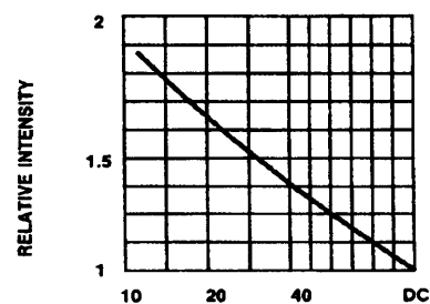
Fig.5 LUMINOUS INTENSITY VS. DUTY CYCLE (AVERAGE I_f=10\text{mA} )
