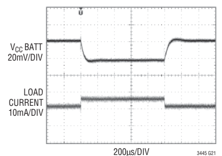
PowerPath LDO Load Step 1mA to 5.5mA
