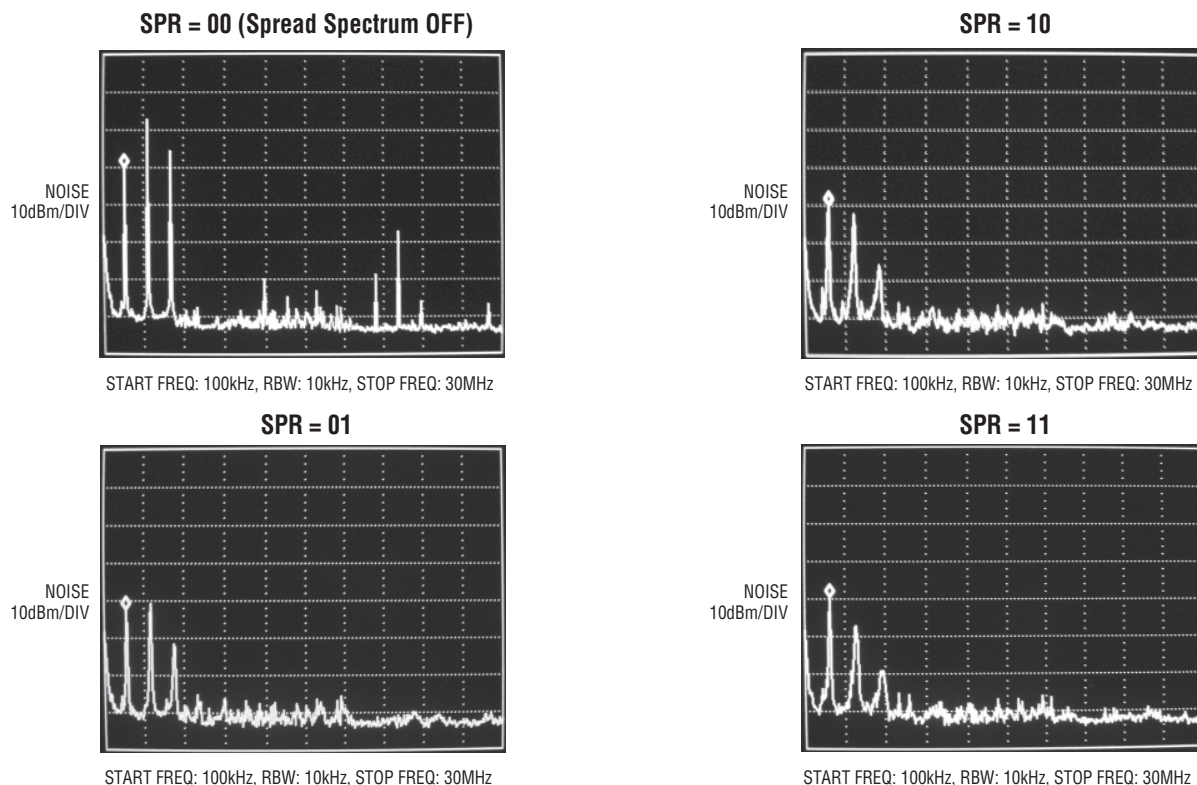
Figure 4. LTC3445 Output Noise Spectrum
