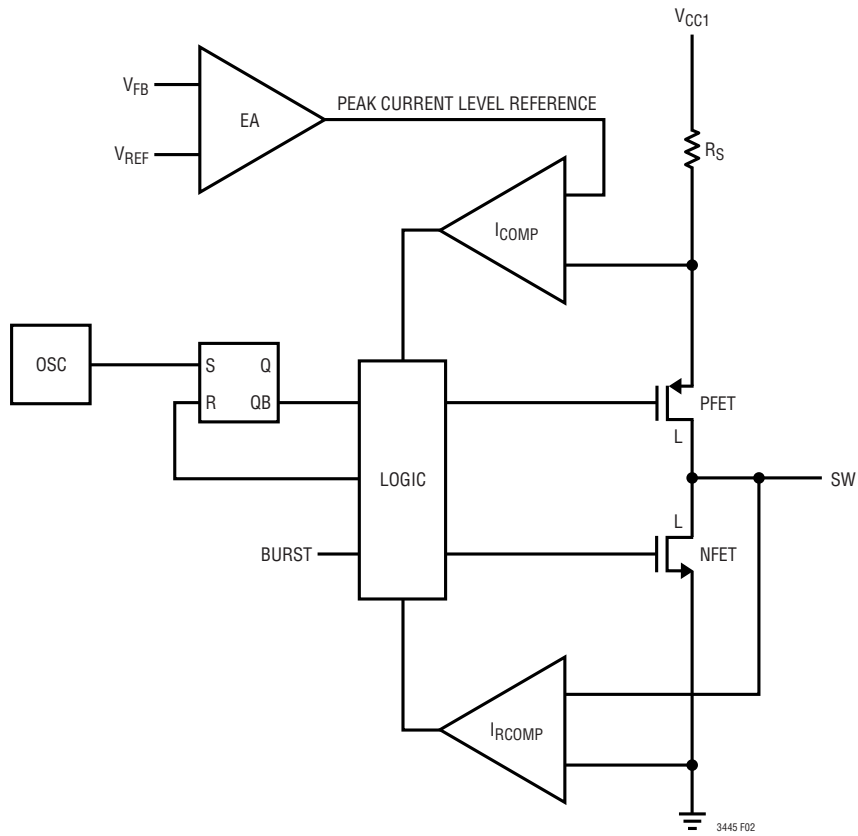
Figure 2. Buck Regulator Detail
