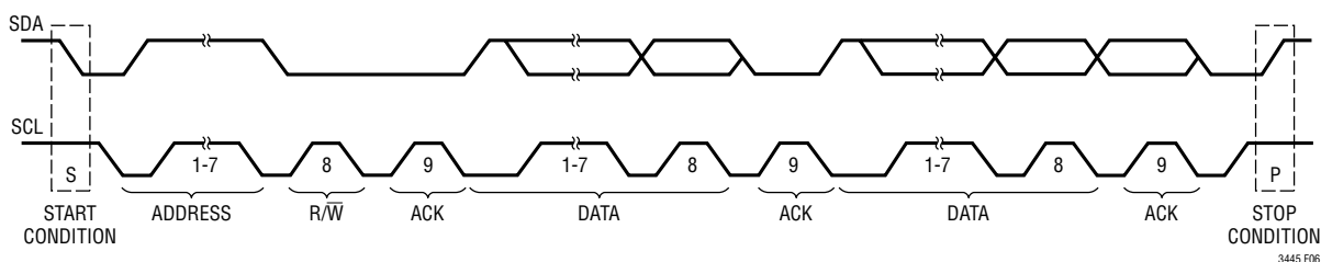
Figure 6. Typical 2-Wire Serial I 2 C Waveforms
