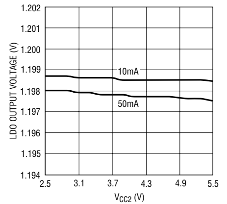
LDO Output Voltage vs V_{CC2}
