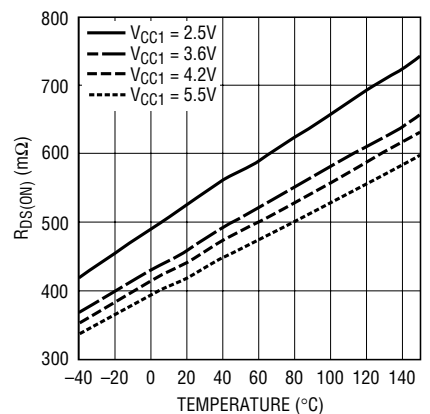
Main Switch R_{DS(ON)} vs Temperature
