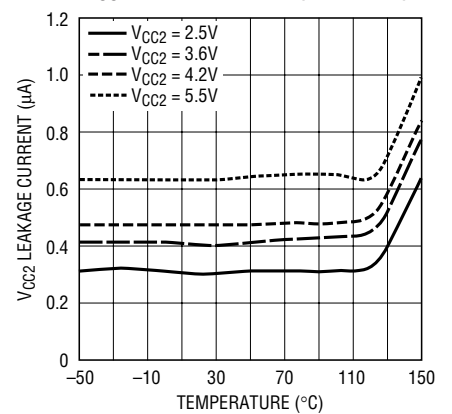
I_{VCC2} vs Temperature (RUN = 0V)
