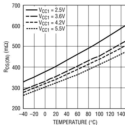
Synchronous Switch R_{DS(ON)} vs Temperature
