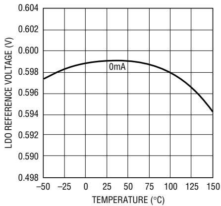
LDO Reference Voltage vs Temperature
