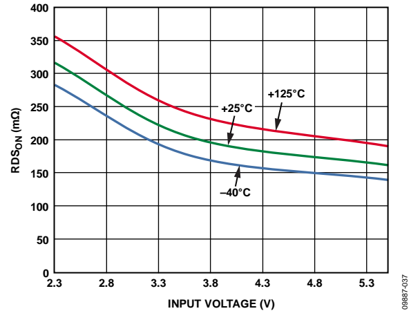
Figure 32. NMOS R_{DS(ON)} vs. Input Voltage Across Temperature
