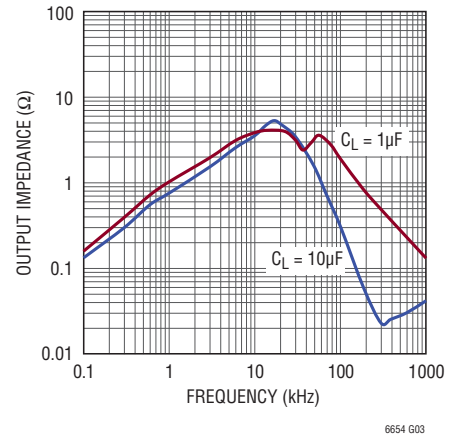
1.25V Output Impedance vs Frequency
