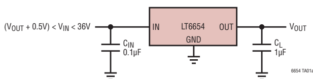
Basic Connection
