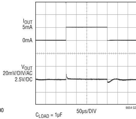
2.5V Load Transient Response (Sinking)
