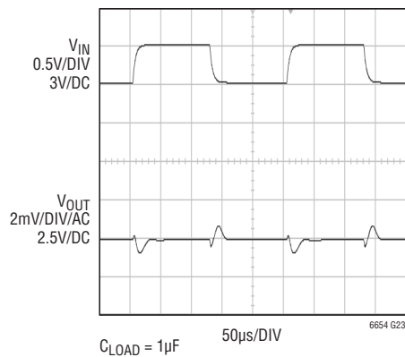
2.5V Line Transient Response
