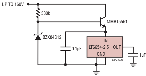
Extended Supply Range Reference
