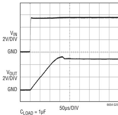
5V Turn-On Characteristics
