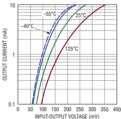
2.5V Minimum V_{IN} to V_{OUT} Differential (Sourcing)
