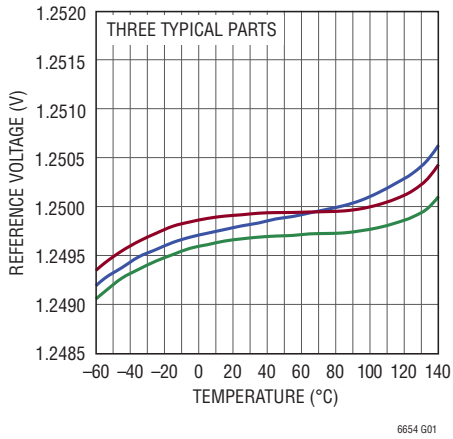
1.25V Output Voltage Temperature Drift
