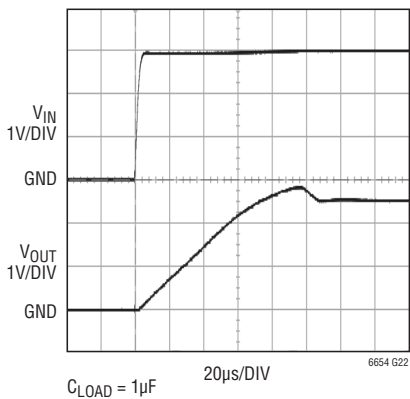
2.5V Turn-On Characteristics
