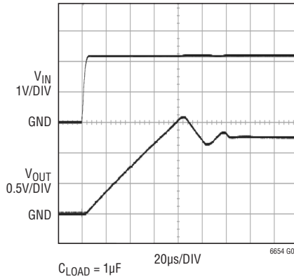
1.25V Turn-On Characteristics
