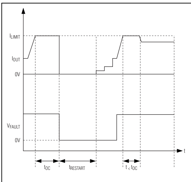
Figure 9. Overcurrent Response
