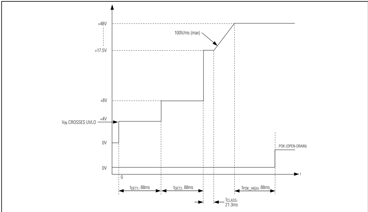
Figure 6. Startup Sequence
