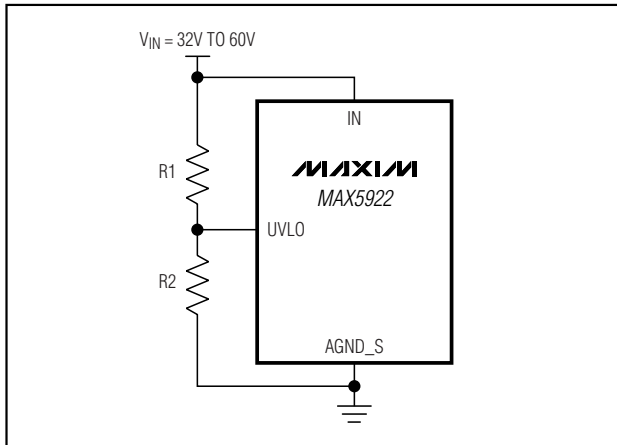
Figure 7. Setting Undervoltage Lockout with an External Resistive-Divider
