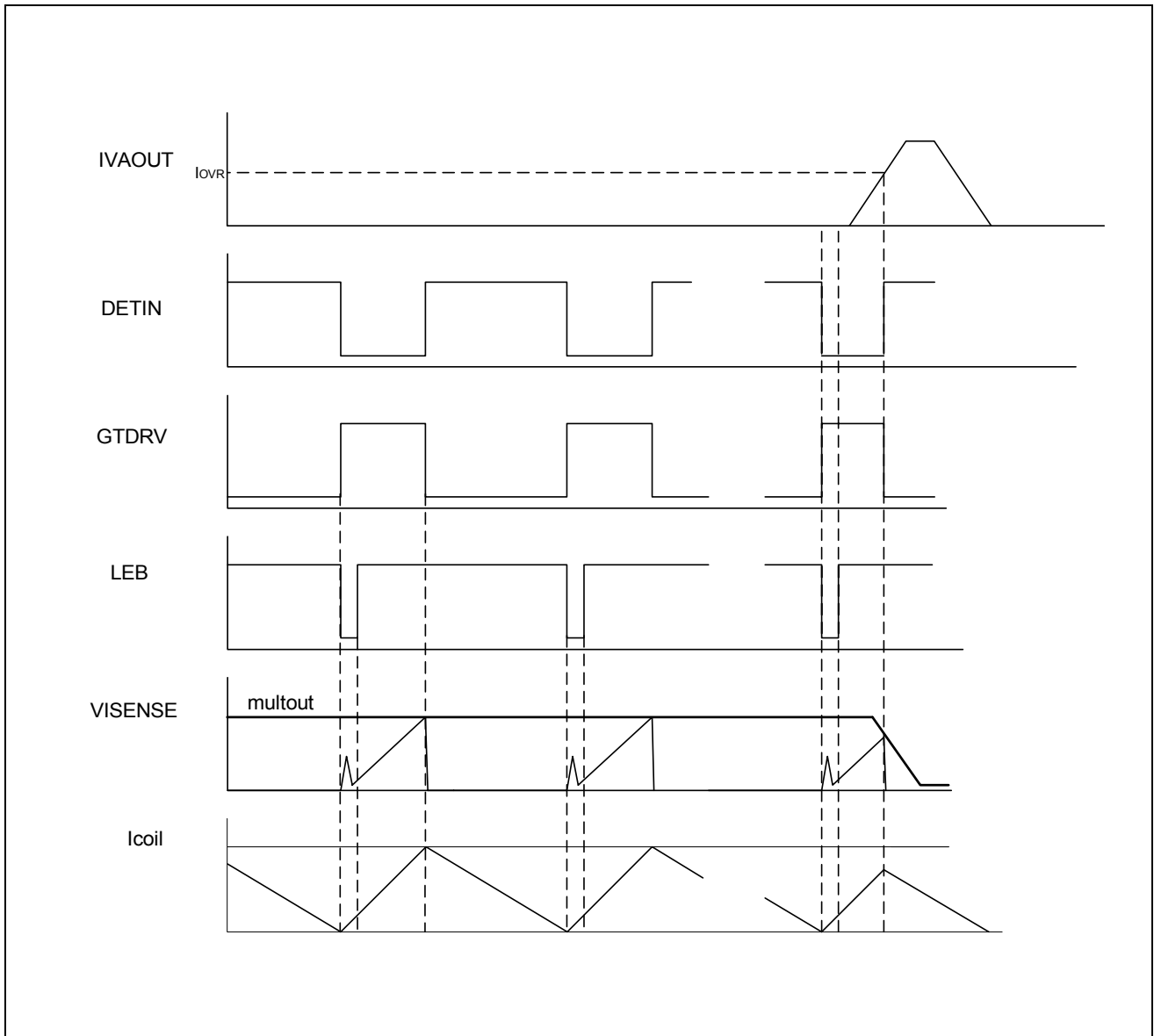
Figure 4 Typical signals
