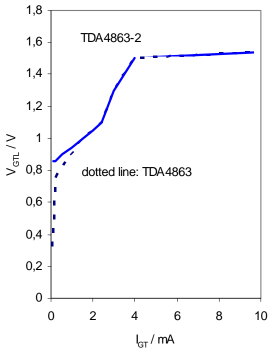
Gate Drive Voltage Low State versus IGT
