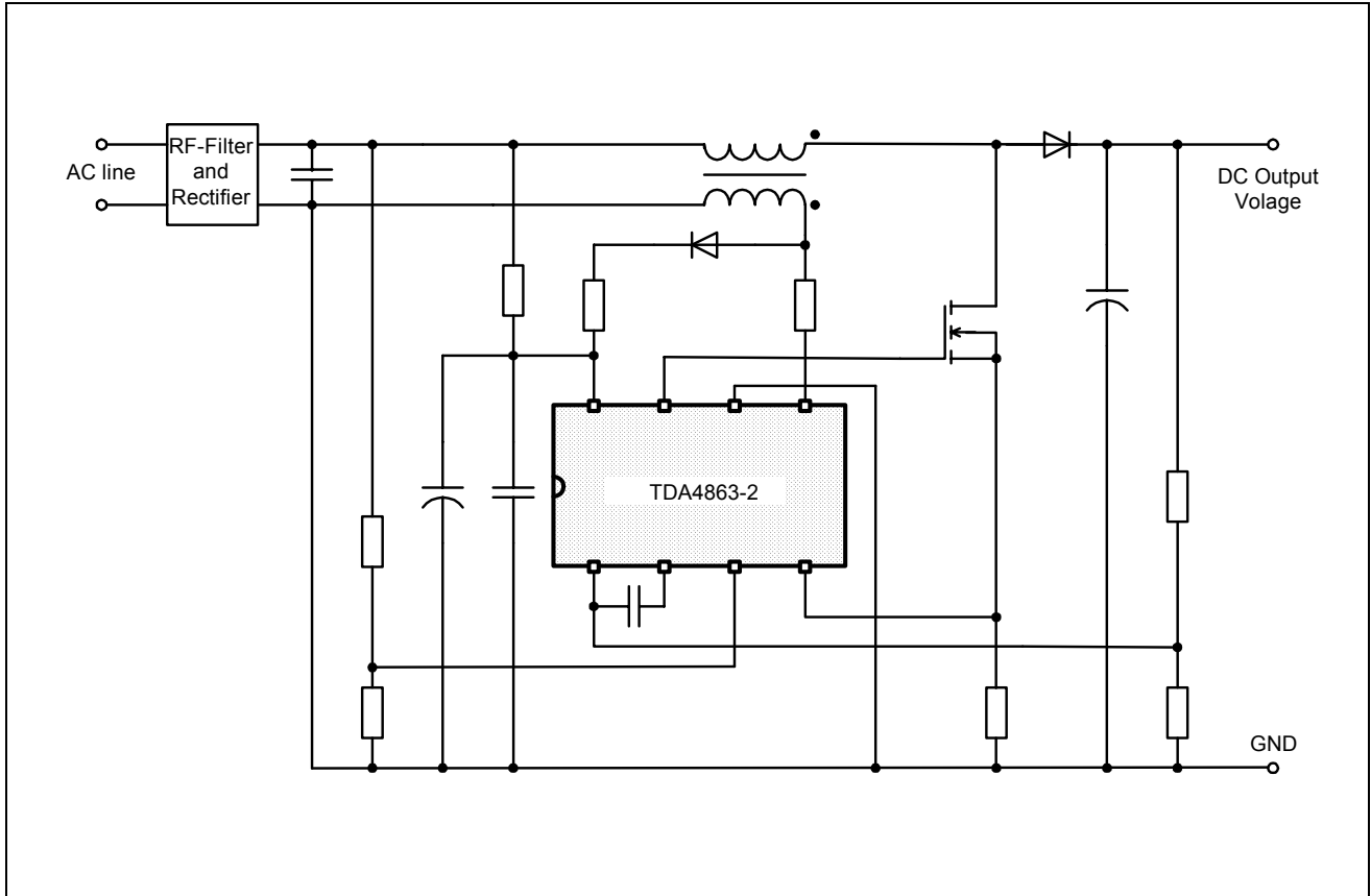
Figure 1 Typical application
