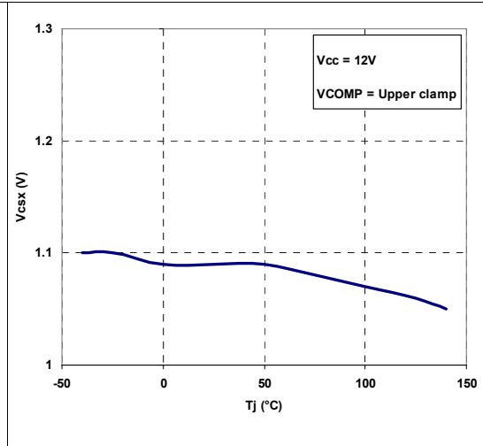
Figure 12. Vcsx clamp vs T J
