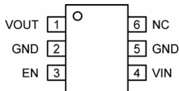
SC-70-6 (C6)
