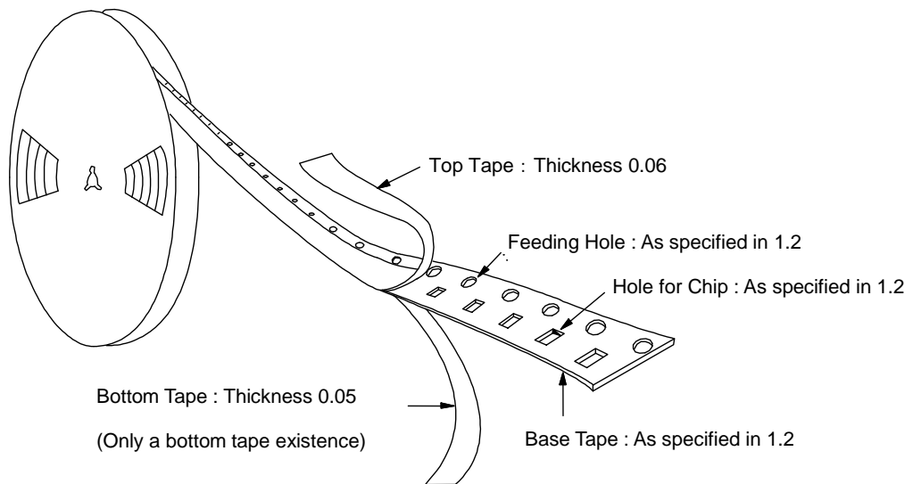
Fig.3 Taping Diagram
