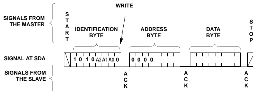
FIGURE 18. BYTE WRITE SEQUENCE
