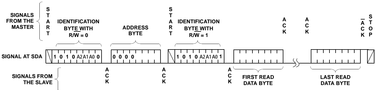
FIGURE 19. READ SEQUENCE
