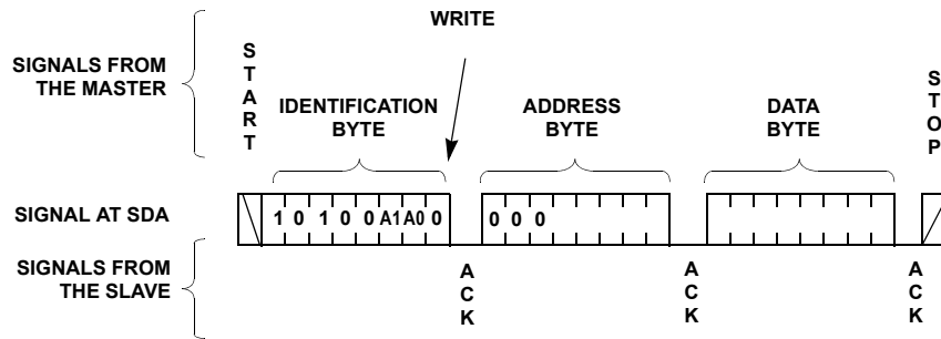
FIGURE 29. BYTE WRITE SEQUENCE
