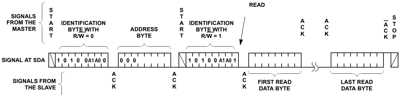
FIGURE 30. READ SEQUENCE
