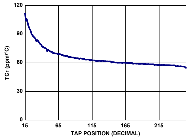
FIGURE 18. 100k TCr vs TAP POSITION
