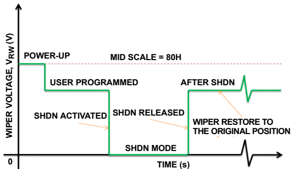
FIGURE 26. SHUTDOWN MODE WIPER RESPONSE
